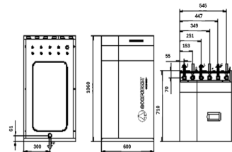
Outdoor unit - AU12
