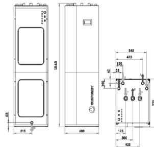
Indoor unit - ecoGEO+ C
