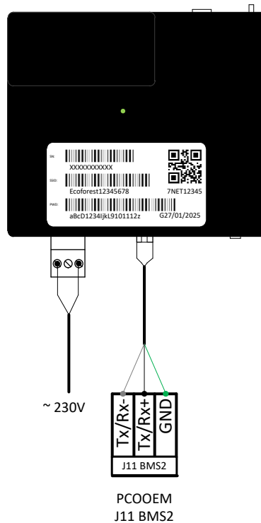
Figure 3.1. Installation of the EASYNET GATEWAY G2 to the ECOFOREST device.
