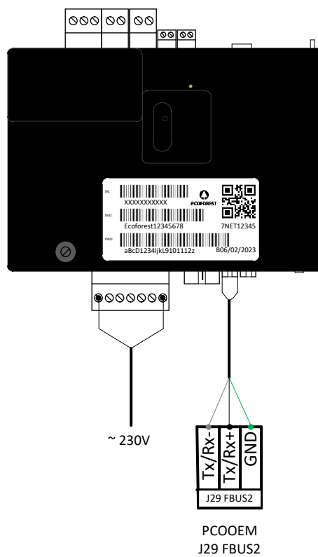
Figure 3.1. Installation of the EASYNET GATEWAY to the ECOFOREST device.
